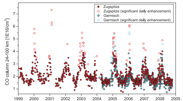
Figure 2. Stratomesospheric CO measured by FTIR at Zugspitze and Garmisch (daily means).
