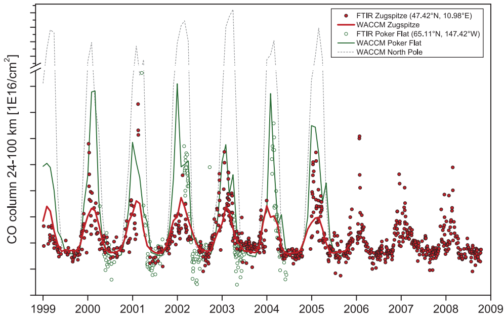
Figure 4. Stratomesospheric CO measured by the Zugspitze FTIR (daily means) and WACCM model results for different latitudes (monthly means). Poker Flat FTIR data were taken from Jones et al. [2007].
