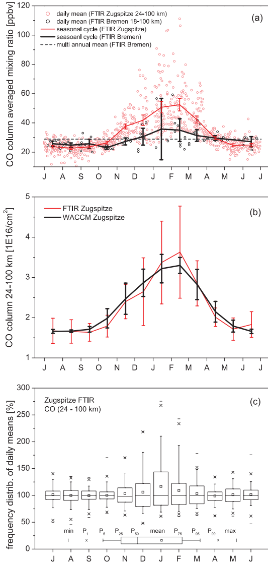
Figure 3. (a) Significance of seasonal cycles (error bars are the 95% confidence statistical errors of the multi-annual monthly means). Bremen data were taken from Velazco et al. [2007, Figure 7]. (b) Inter-annual variability (1-sigma bars) on the monthly scale. (c) Frequency distributions of Zugspitze FTIR daily means in percent of the multi-annual median (P are percentiles).
