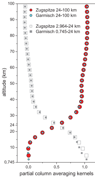
Figure 1. Characterization of the optimized FTIR retrieval of stratomesospheric CO at mid-latitudes. Mean averaging kernels for all states measured in 2004–2008.
