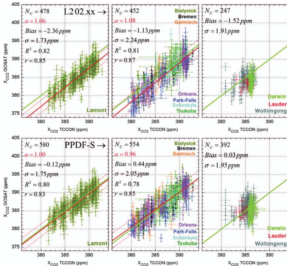
Fig. 6. Correlation diagrams between GOSAT and ground-based TCCON measurements of X_{CO_2} for two GOSAT retrieval algorithms, PPDF-S (bottom panels) and NIES L2 02.xx (top panels), and for three sets of TCCON sites, over Lamont (left-hand panels), over the other seven Northern Hemisphere sites (middle panels), and over three Southern Hemisphere sites (right-hand panels). The GOSAT single scans were selected during 14 months from June 2009 within a 5^\circ radius latitude/longitude circle centered over each TCCON station. The analyzed ground-based FTS data were mean values measured within \pm 1 h of the GOSAT overpass time. Red lines correspond to the best fits, and the green line represents one-to-one correspondence. The number of coincident soundings and characteristics of statistical relationships between ground-based FTS and GOSAT X_{CO_2} for each set of TCCON stations is listed in the legend of each panel.
